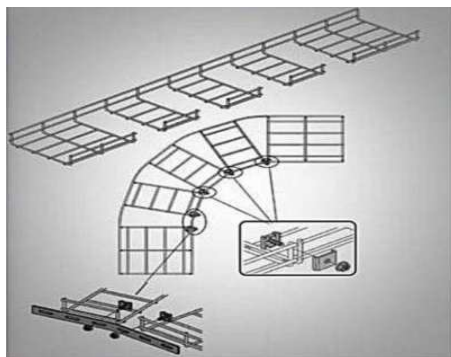
Elbow Long 90 Degree
