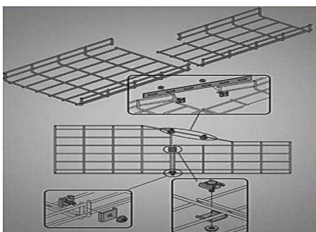
Reducer With Joint
