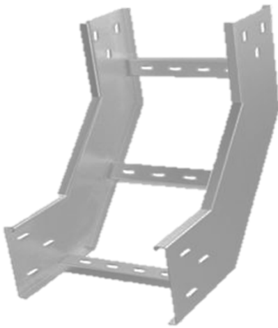
RISER (INSIDE/OUTSIDE) TYPE RADIUS/DIAGONAL
